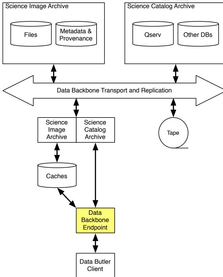
FIGURE 3: The Data backbone links all the physical components of DM.
