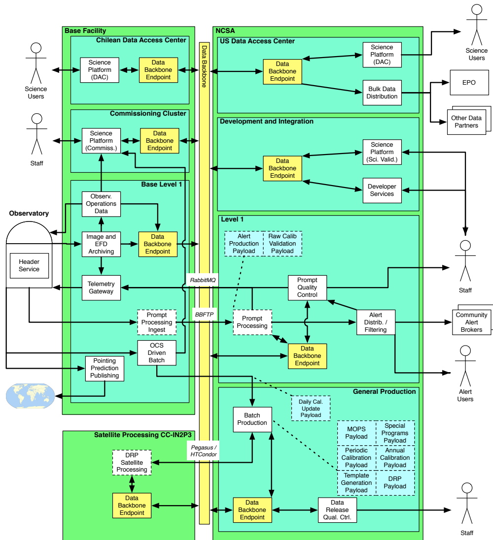
FIGURE 1: DM components as deployed during Operations. Where components are deployed in multiple locations, the connections between them are labeled with the relevant communication protocols. Science payloads are shown in blue.
