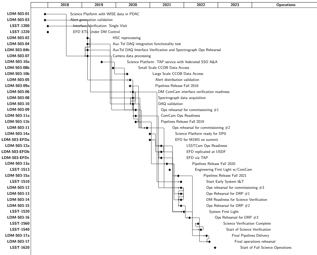
FIGURE 9: DM major milestones—designated as LDM-503-x—in the LSST schedule. These milestones are defined at level 2 according to the scheme described in Section 4.3.
