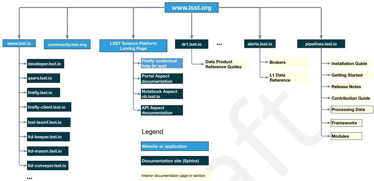
FIGURE 7: Outline of the web hierarchy for the DM end user documentation.
